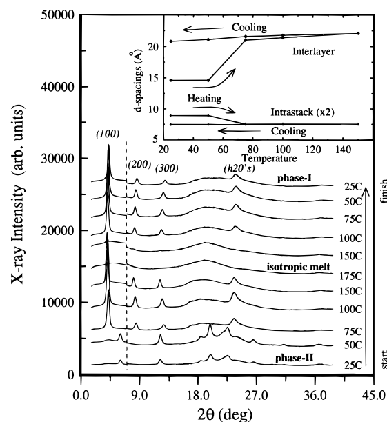
Figure 3. X-ray diffraction profiles of R-P3OT at various temperatures demonstrating the solid-state phase change from the type-II to the type-I structure well below the isotropic melt. Inset: The measured interlayer and intrastack d -spacings of R-P3OT as a function of temperature.
